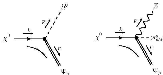
Figure 2. Feynman diagrams for the decay of a Higgsino neutralino into neutral Higgs or gauge bosons and gravitino.
